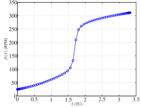
(b) Example 3 Control Using RPM and N = 64 .
